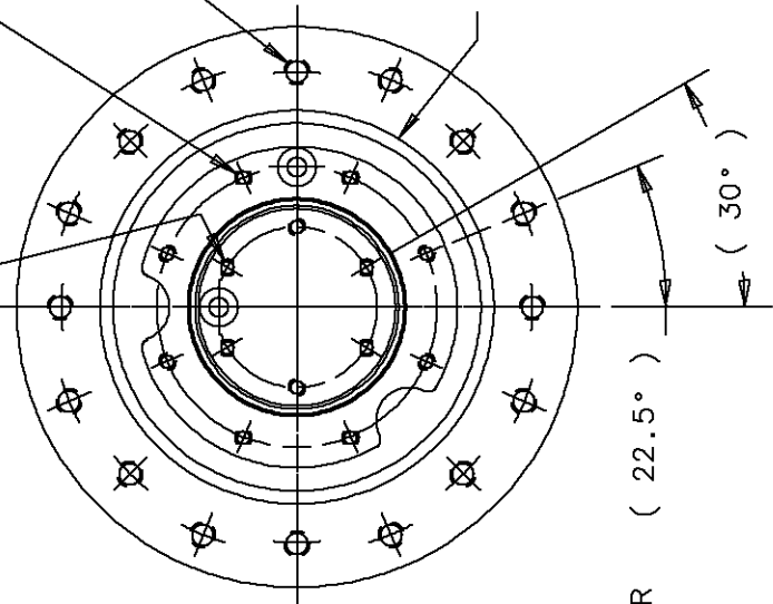
VIEW Z-Z
